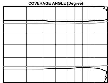
Horizontal (dark) and vertical (light) coverage angles between -6 dB points: cardioid mode.
