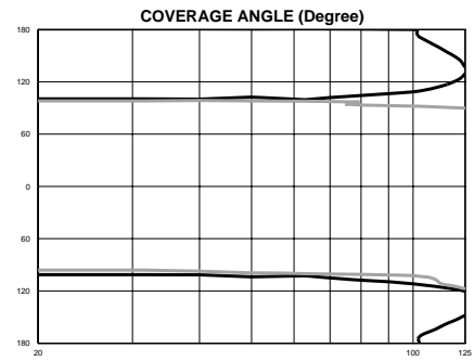
Horizontal (dark) and vertical (light) coverage angles between -6 dB points: supercardioid mode.
